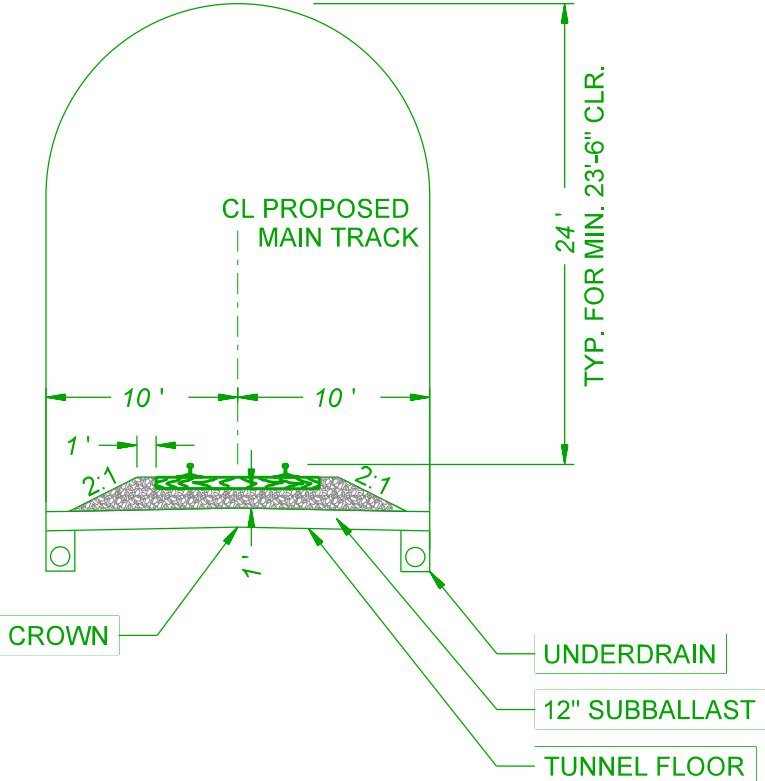
TYPICAL SECTION - TUNNEL (THOREAU OPTION)
