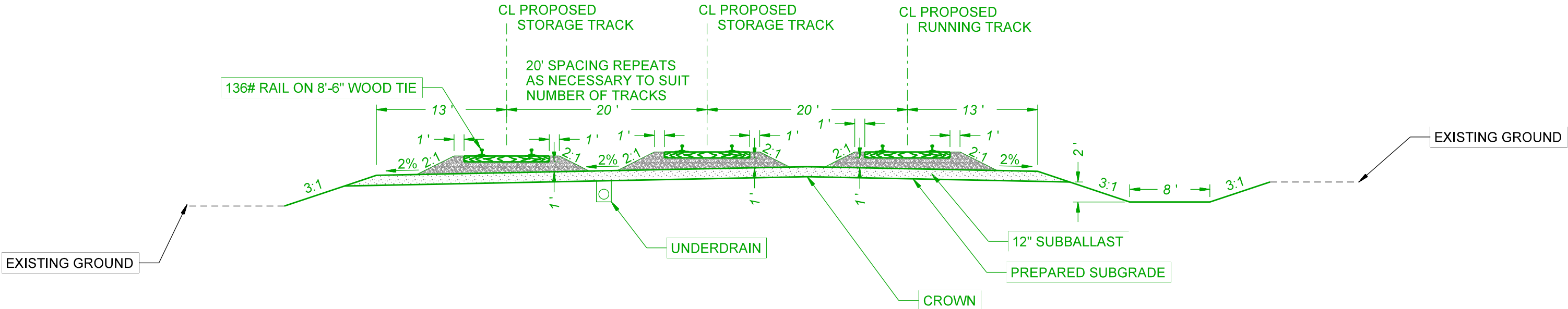
TYPICAL SECTION - MULTIPLE YARD TRACKS
